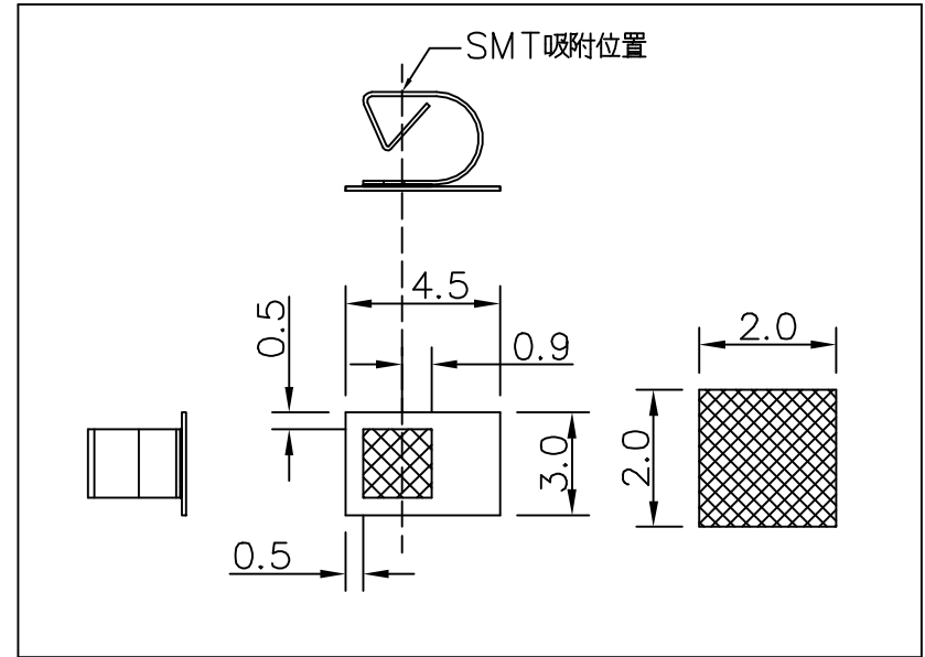
PCB Recommend Layout Pattern
